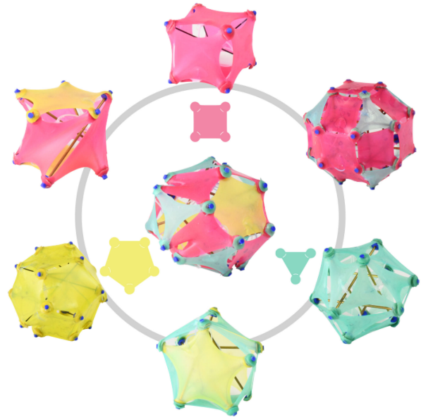
Fig. 1. With square, triangle, and pentagon-shaped membrane actuators as building blocks, we can construct a variety of polyhedra tensegrities. Based on their face arrangement and shapes, tensegrities may be created to more accurately roll on specified paths.
