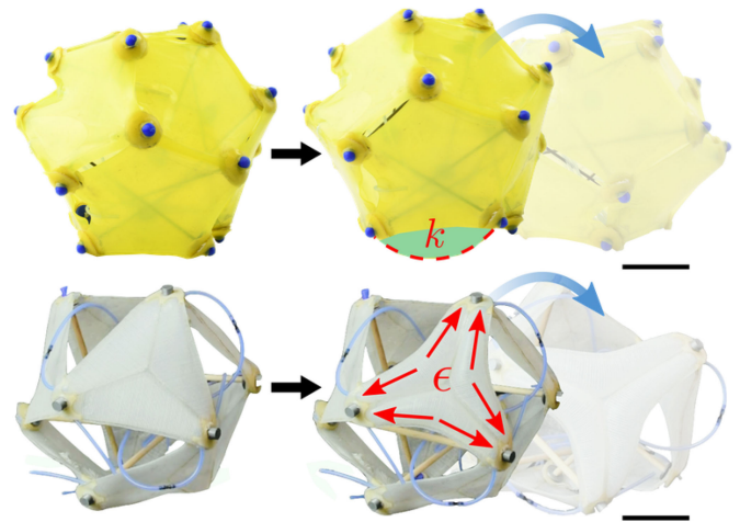
Fig. 4. Rolling mechanisms for tensegrities with out-of-plane expanding membrane actuators, which minimally shift the struts (top dodecahedron), and extension membrane actuators, which significantly shift the struts (bottom icosahedron). Scale bars: 25 mm (top), 40 mm (bottom).
